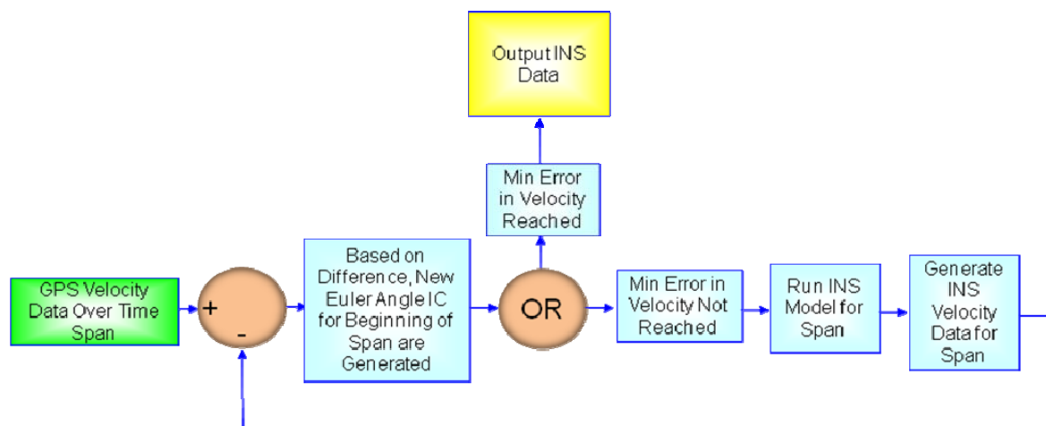
Figure 15. Euler IC GPS correction algorithm
