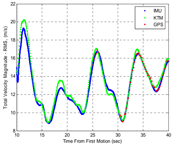
Figure 18. PDPAS velocity solution of a PRS (zoomed in)
